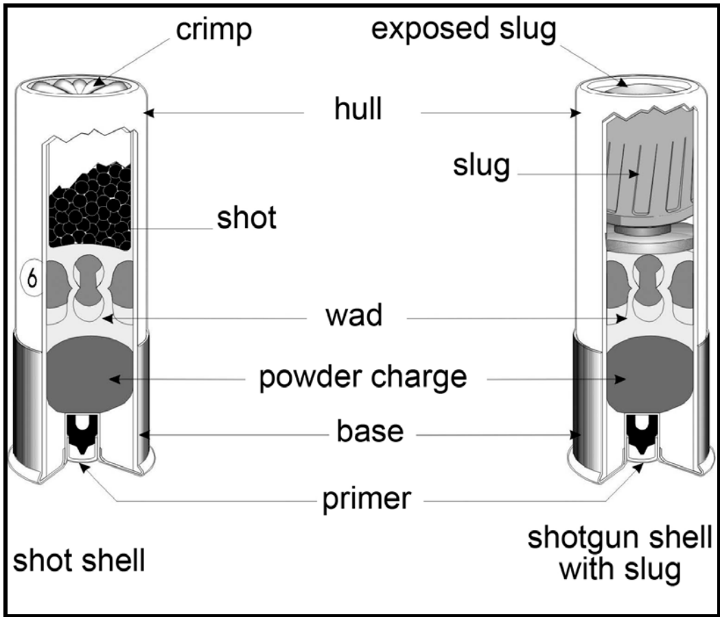
Figure 32. Shotgun Shells
