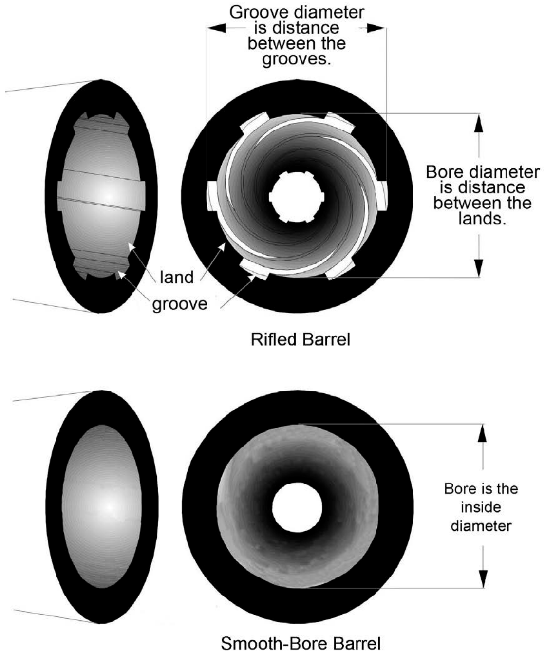
Figure 19. Rifled bore and smooth bore
