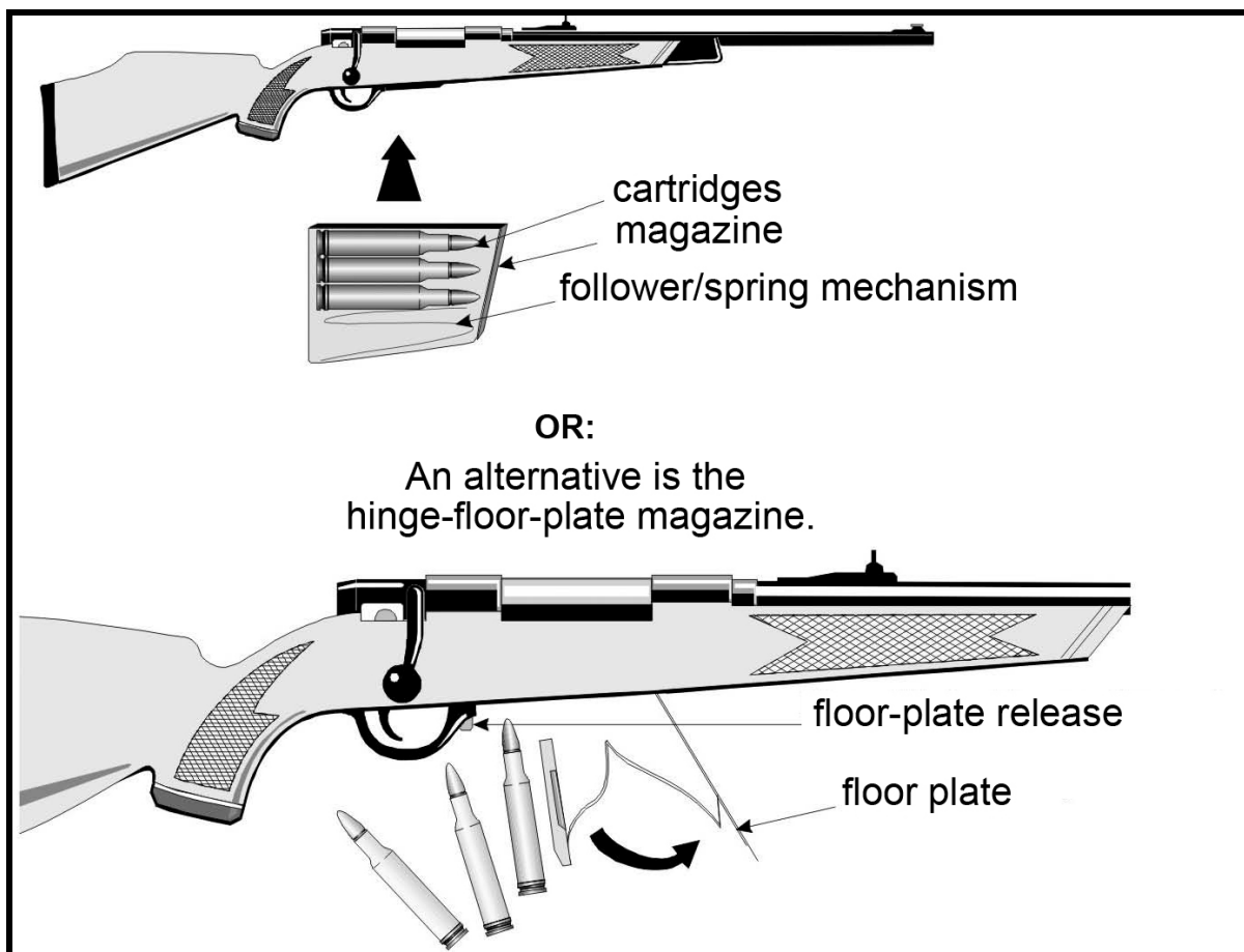
Figure 49. Box-type magazine
